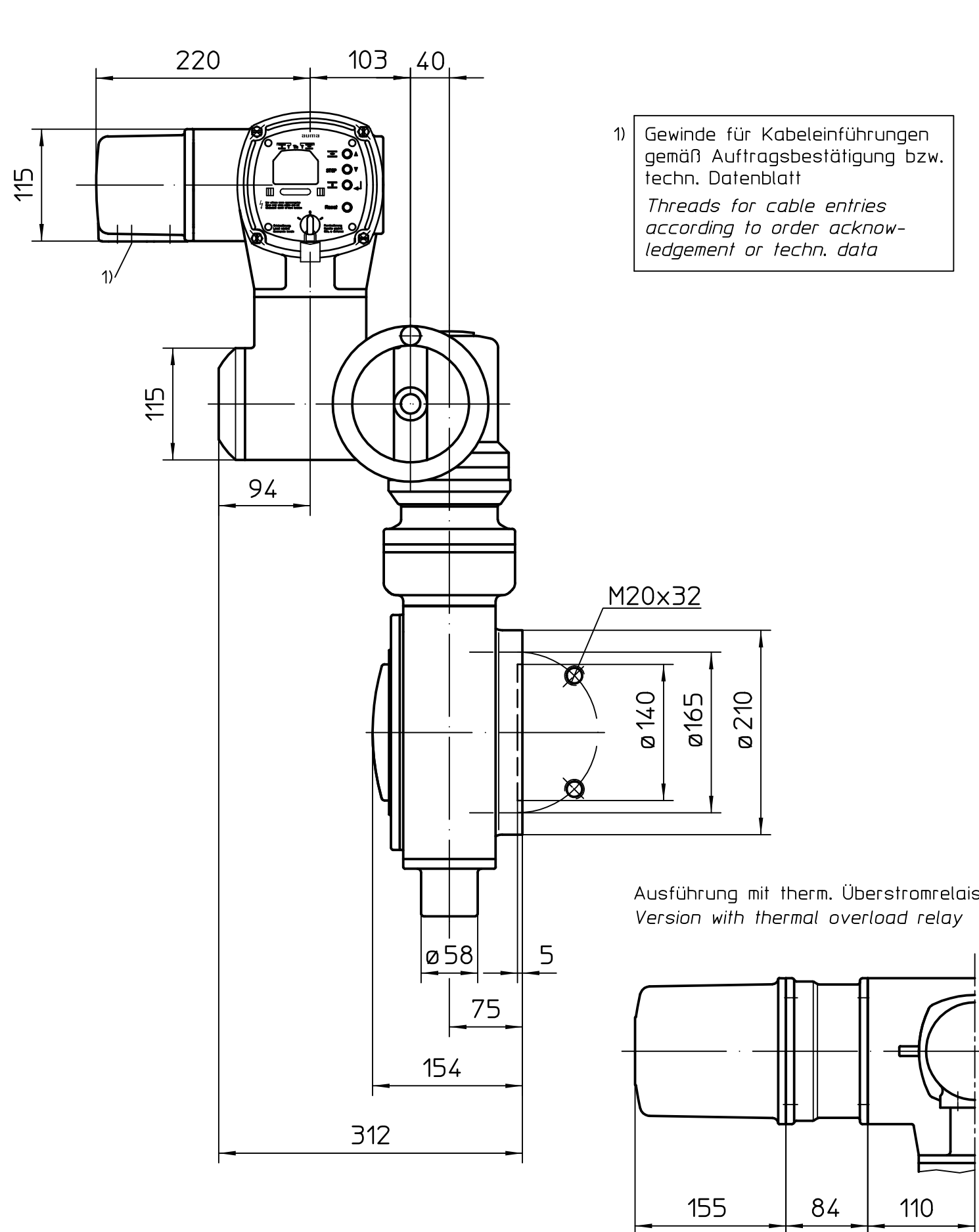
Montage-Position A/Mounting position A
