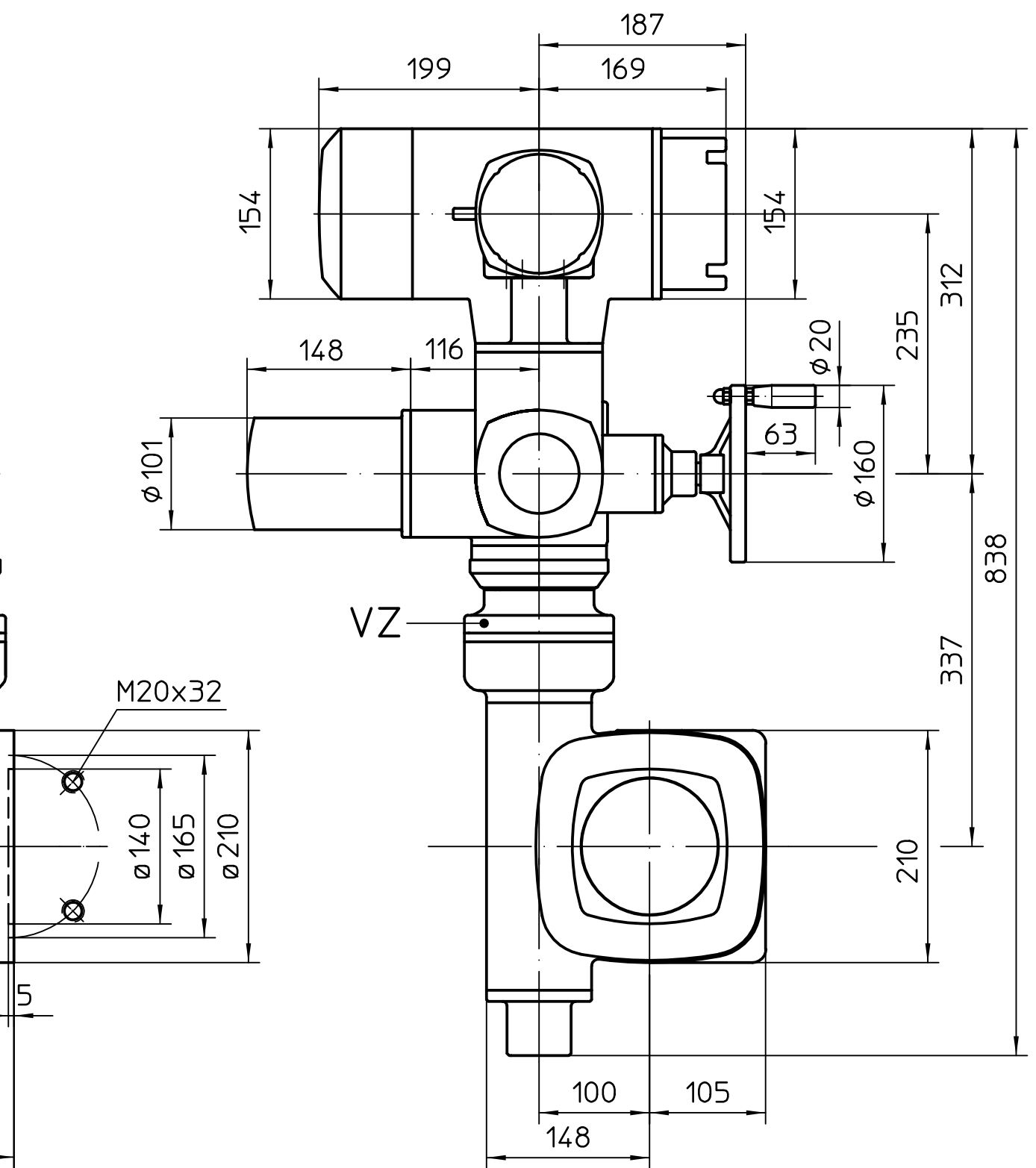
Montage-Position A/Mounting position A
