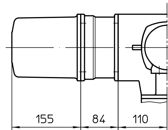
Montage-Position A/Mounting position A
