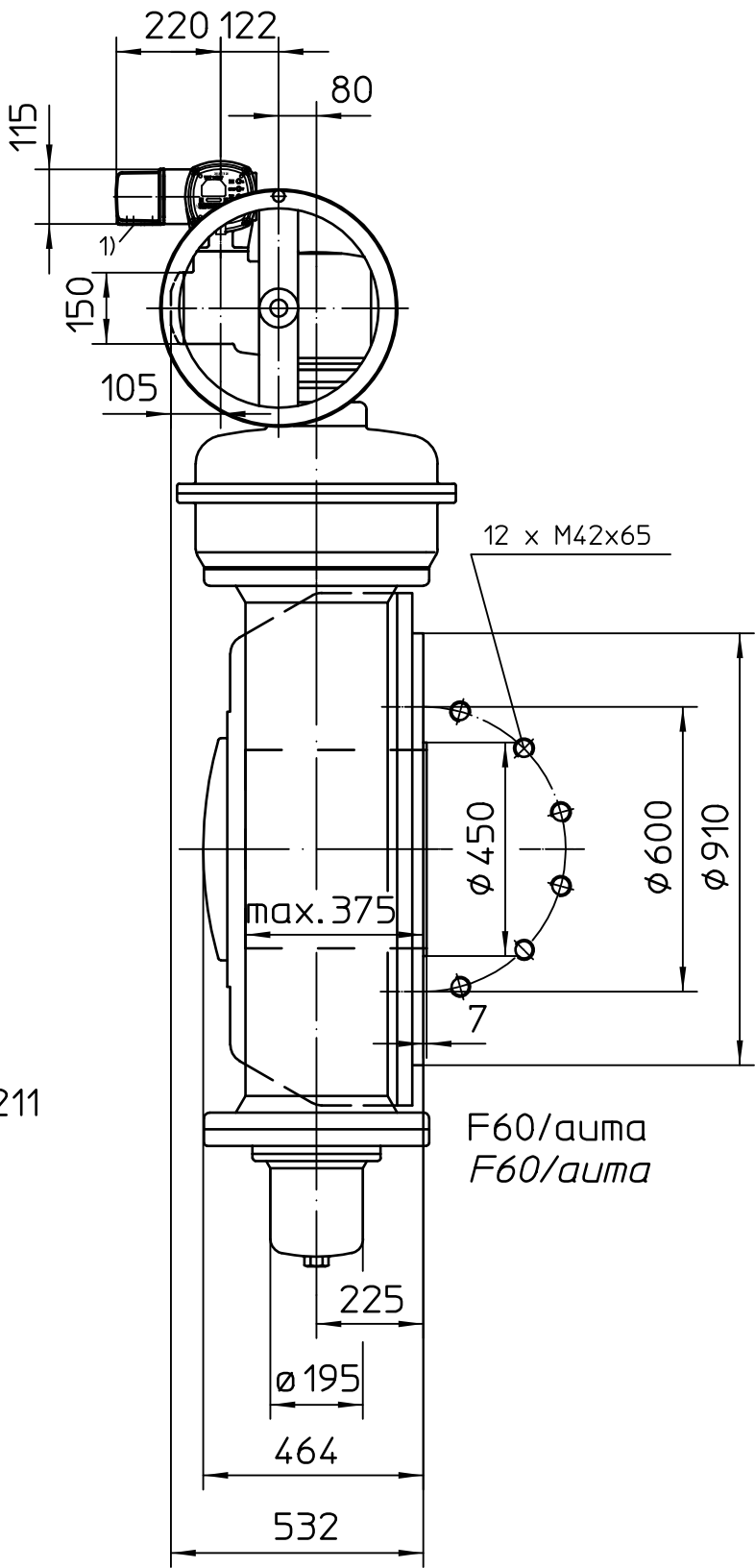
Montage-Position A/Mounting position A
