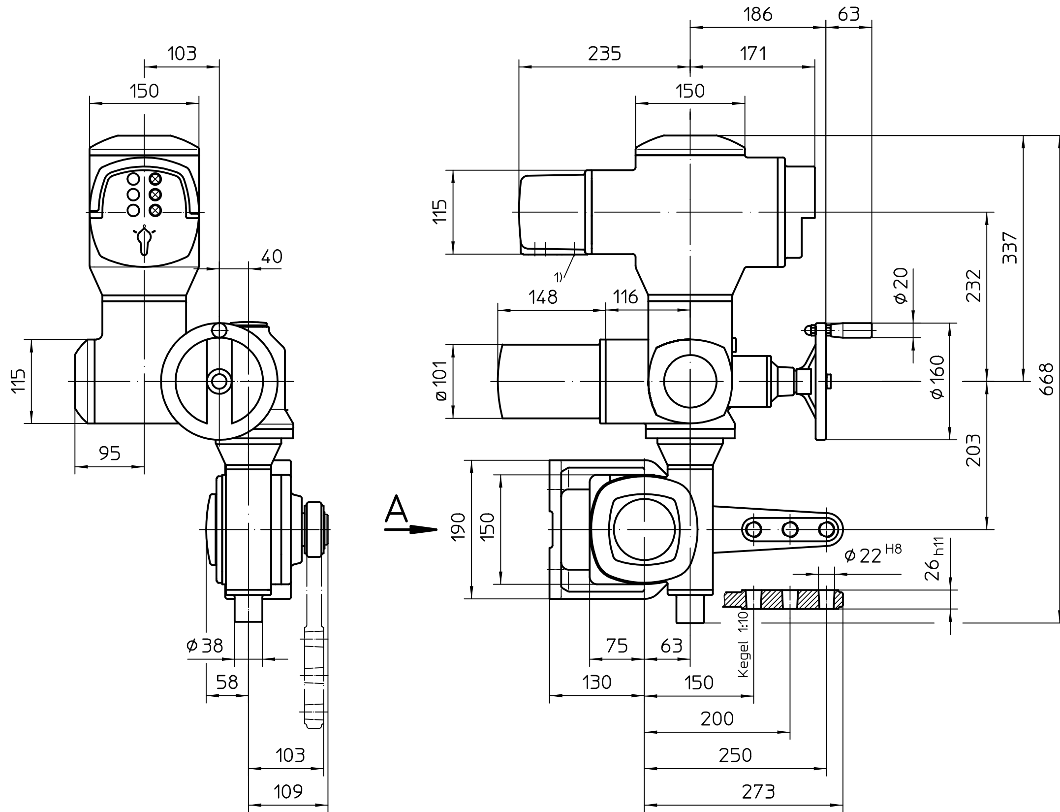
Montage-Position A/Mounting position A
