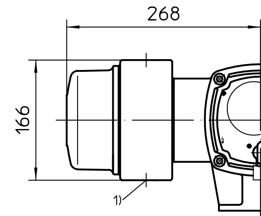
Version KM Exe
