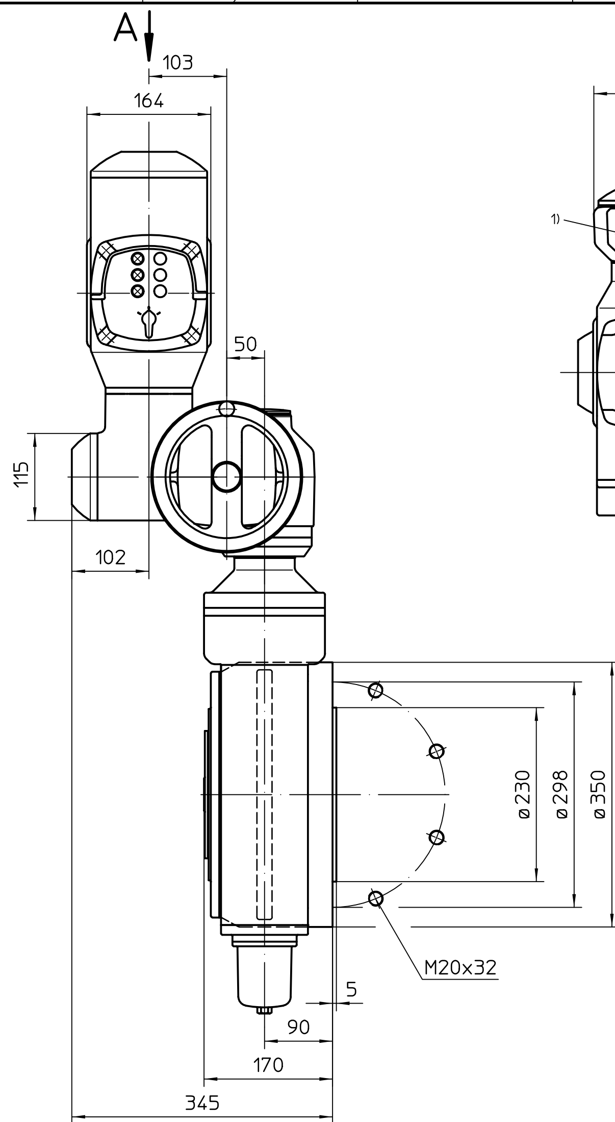
Option Flansch plan
