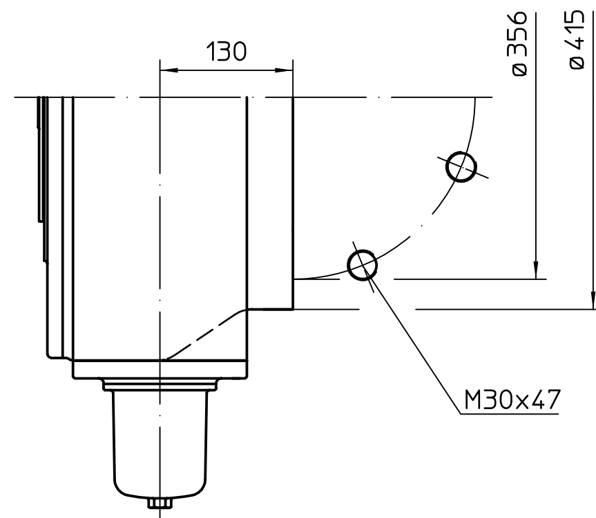
Option Flansch plan
