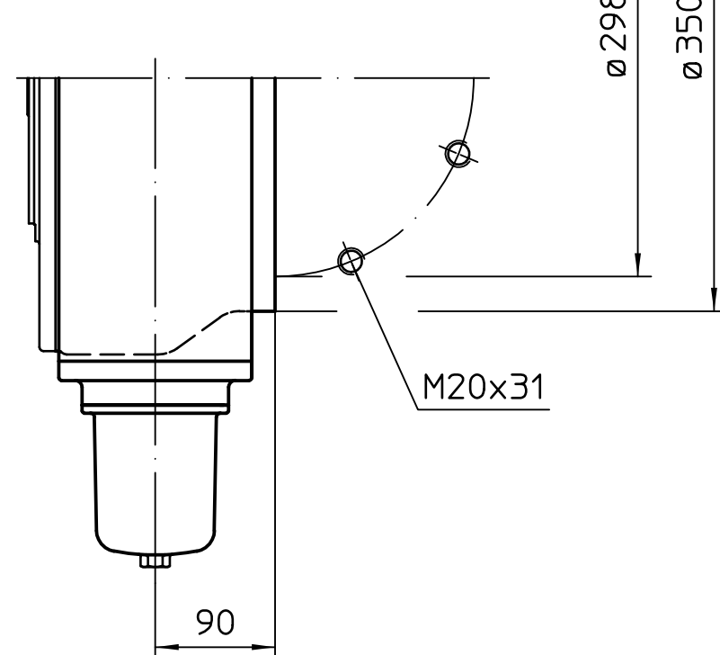
Option Flansch plan
