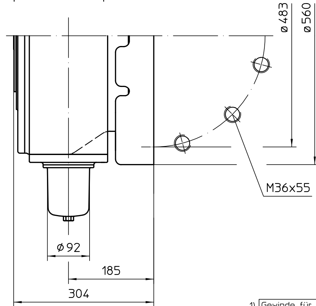
Option Flansch plan
