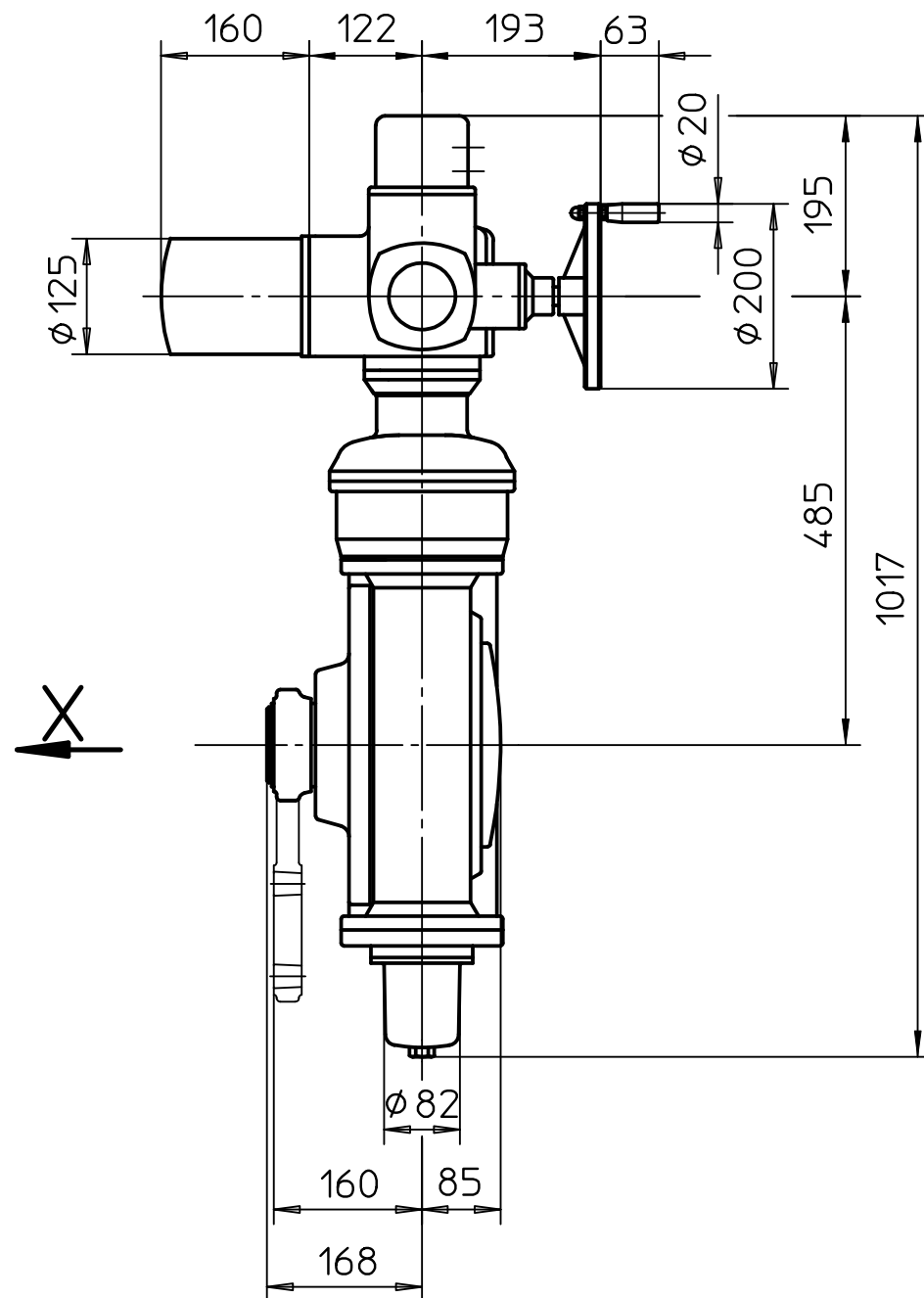
Montage-Position B/Mounting position B
