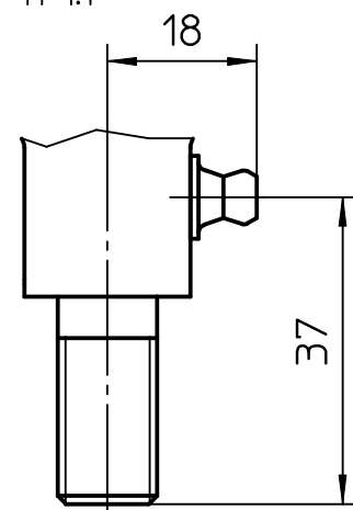
Detail X
