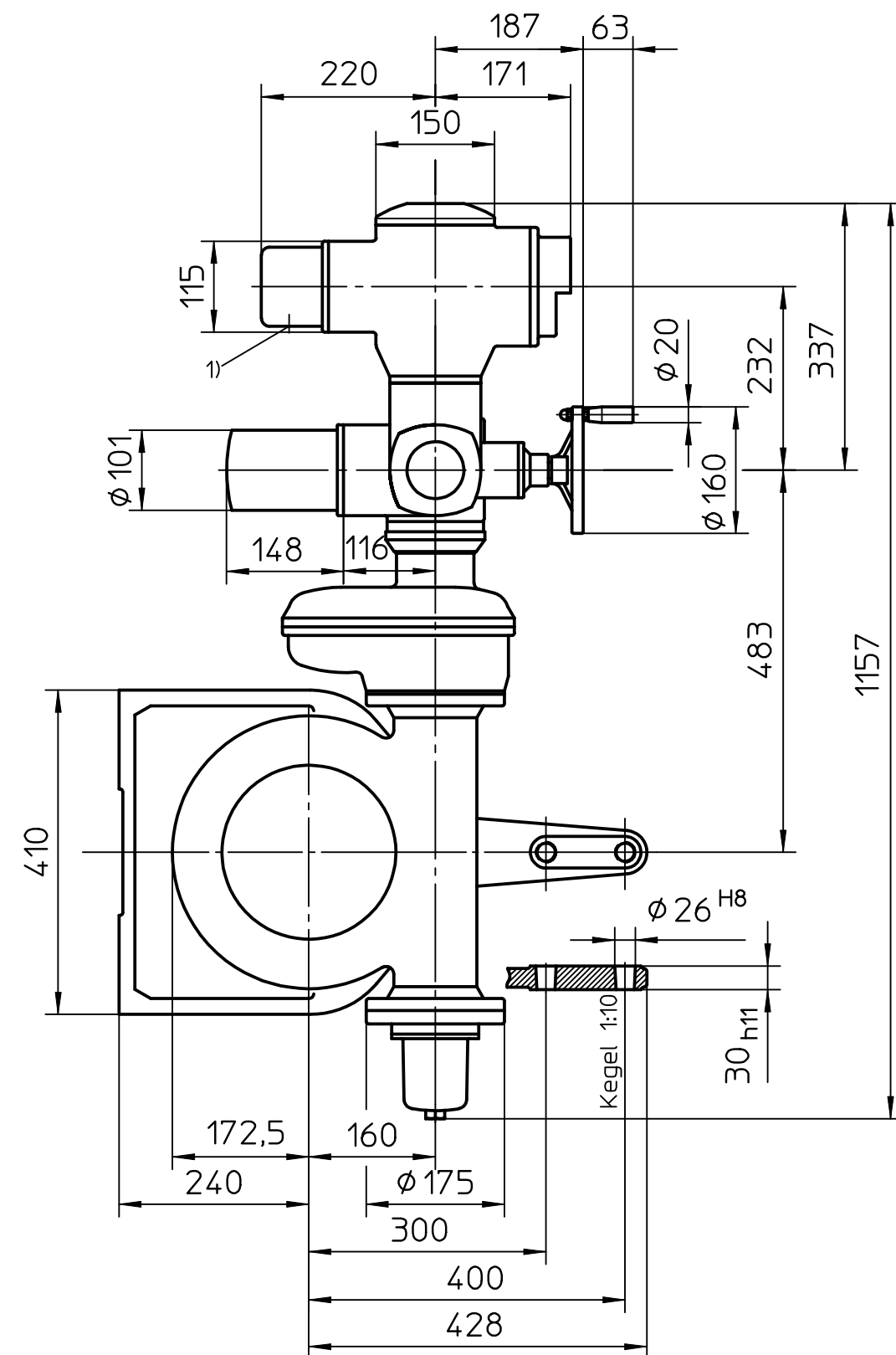
Montage-Position A/Mounting position A
