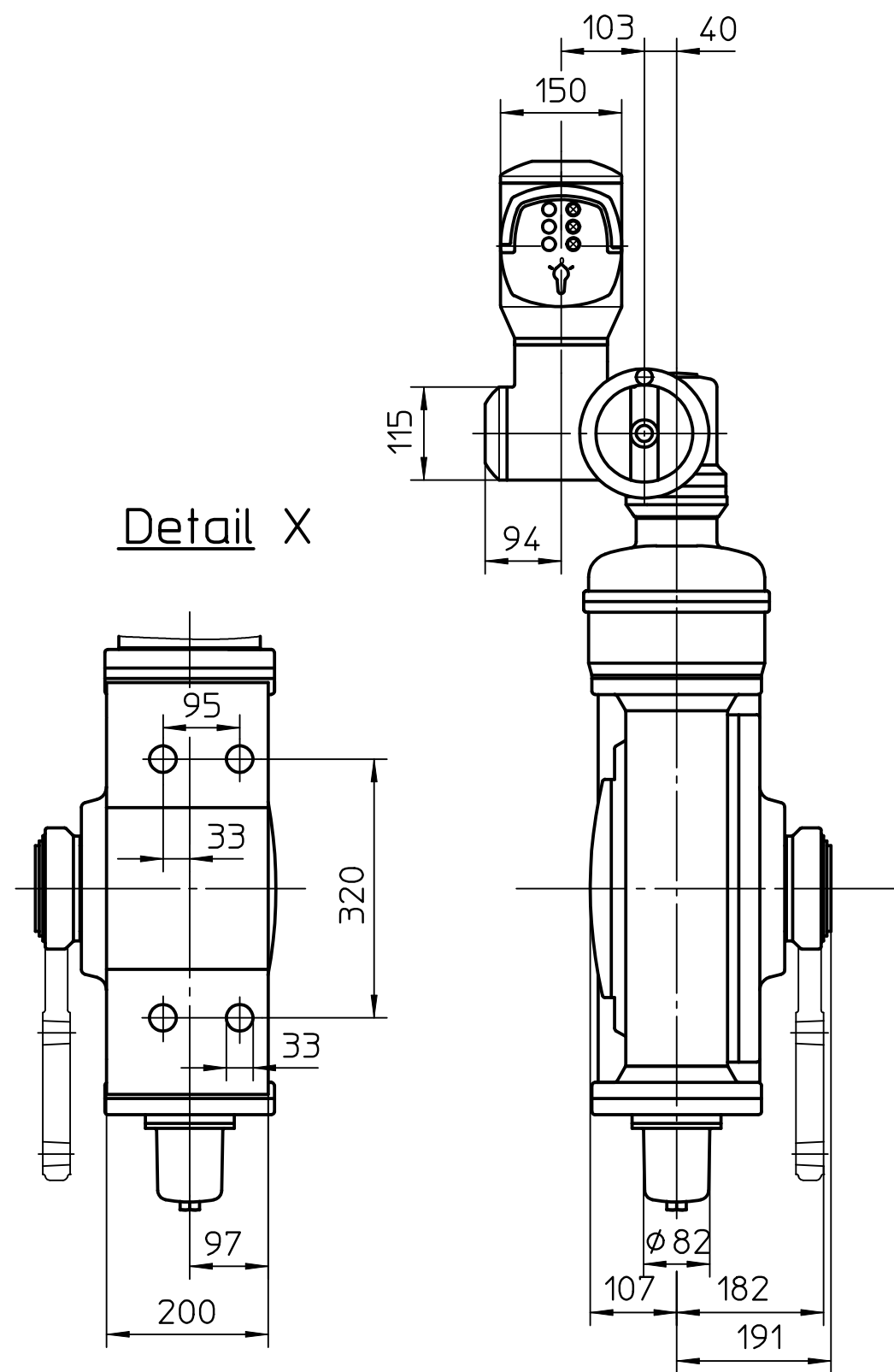
Montage-Position A/Mounting position A
