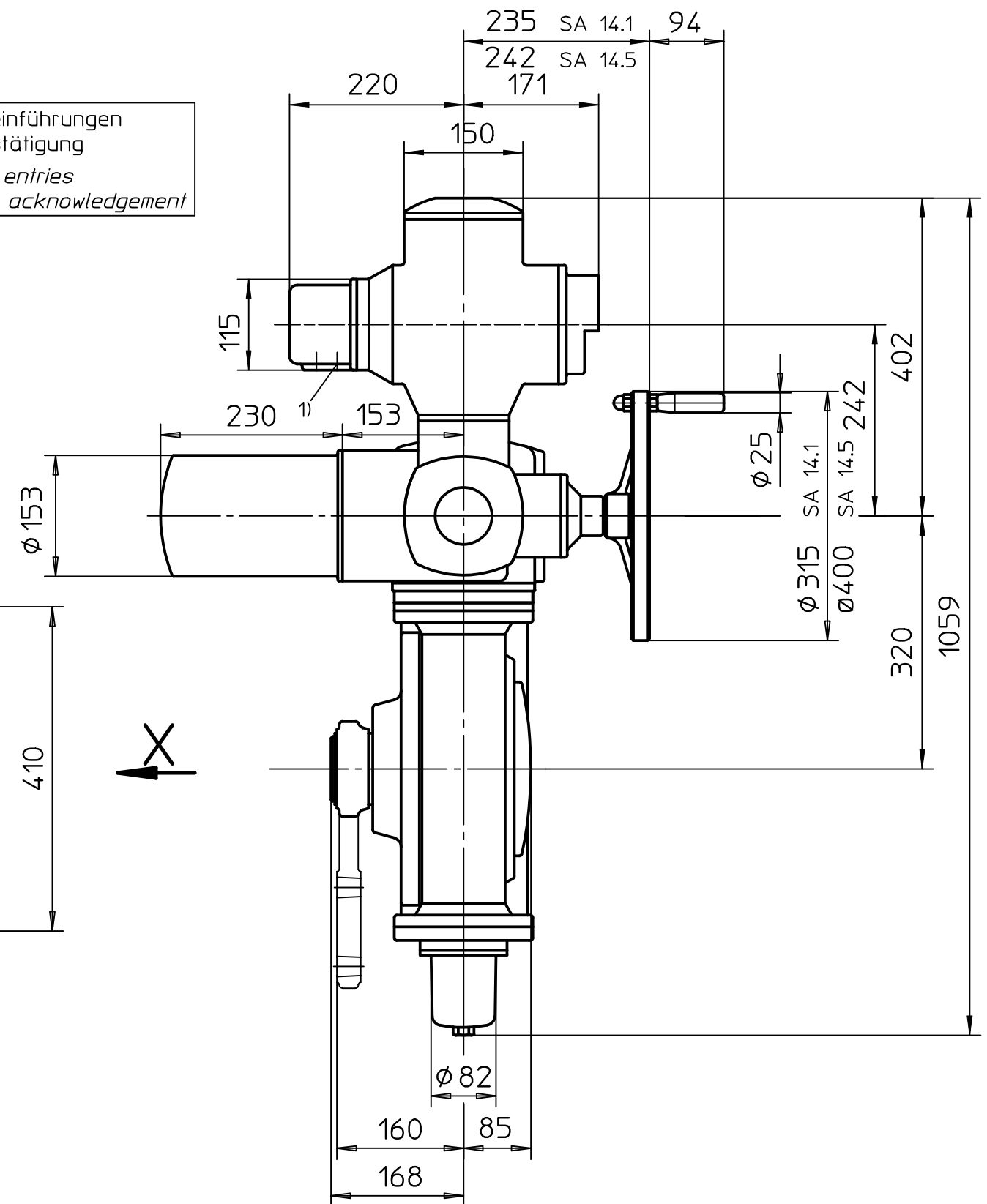
Montage-Position B/Mounting position B
