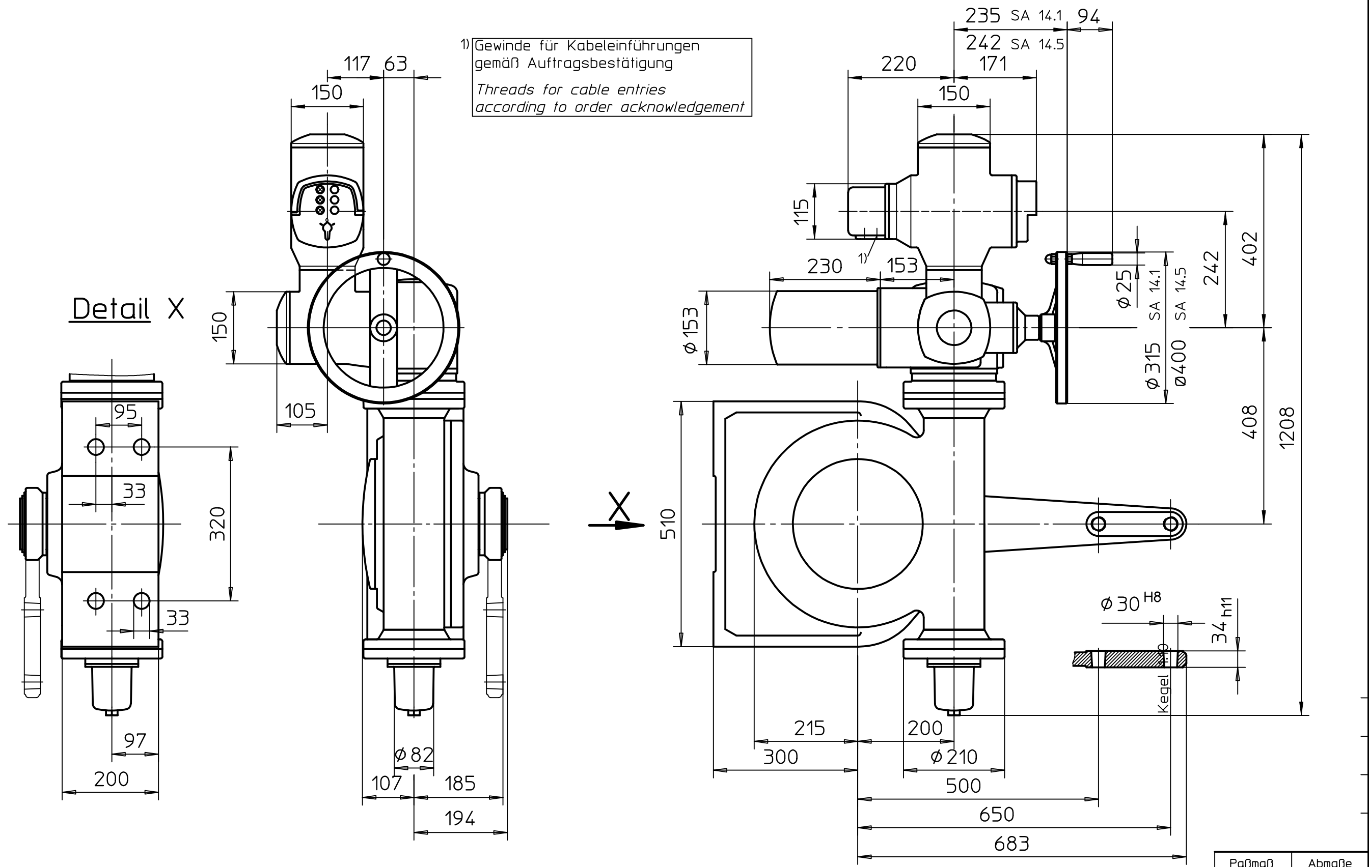
Montage-Position A/Mounting position A
