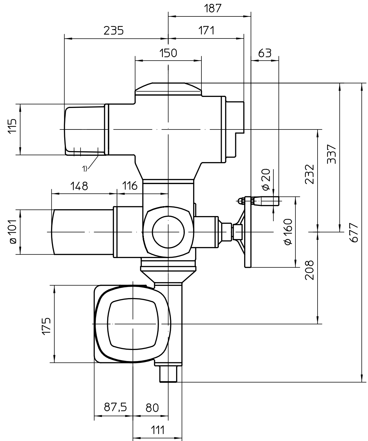
Montage-Position A/Mounting position A
