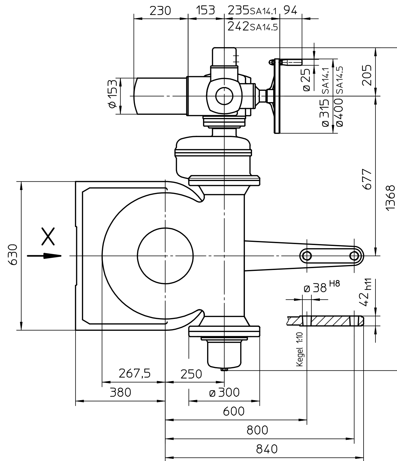
Montage-Position A/Mounting position A
