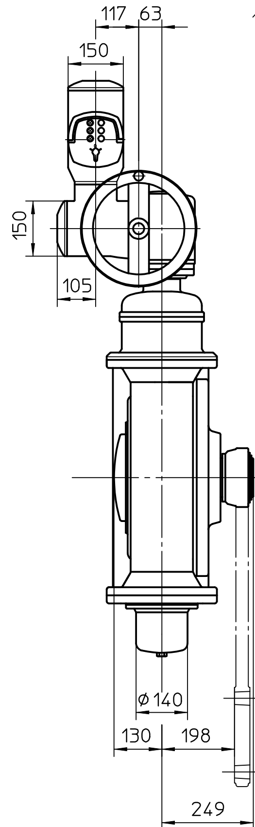
Montage-Position A/Mounting position A
