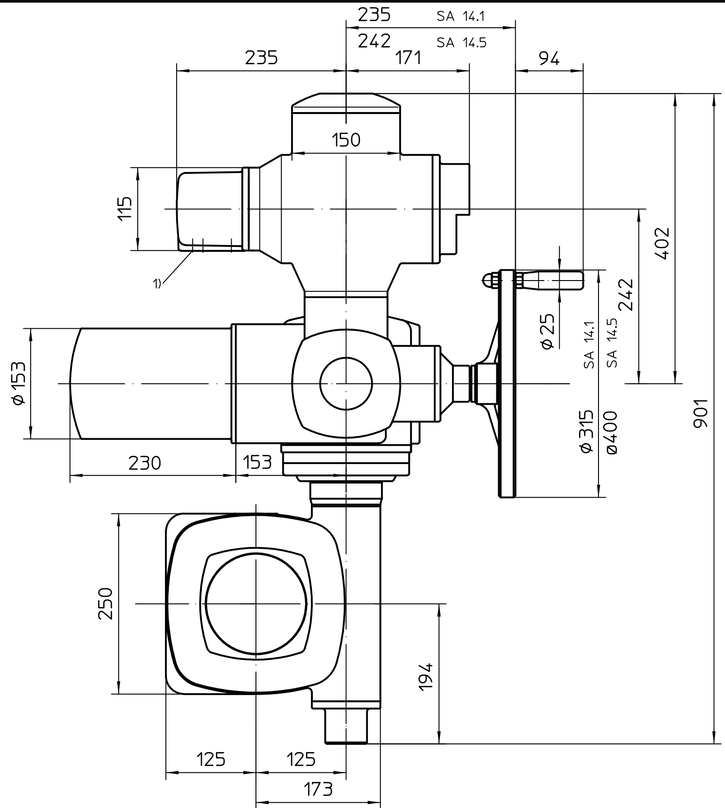
Montage-Position A/Mounting position A
