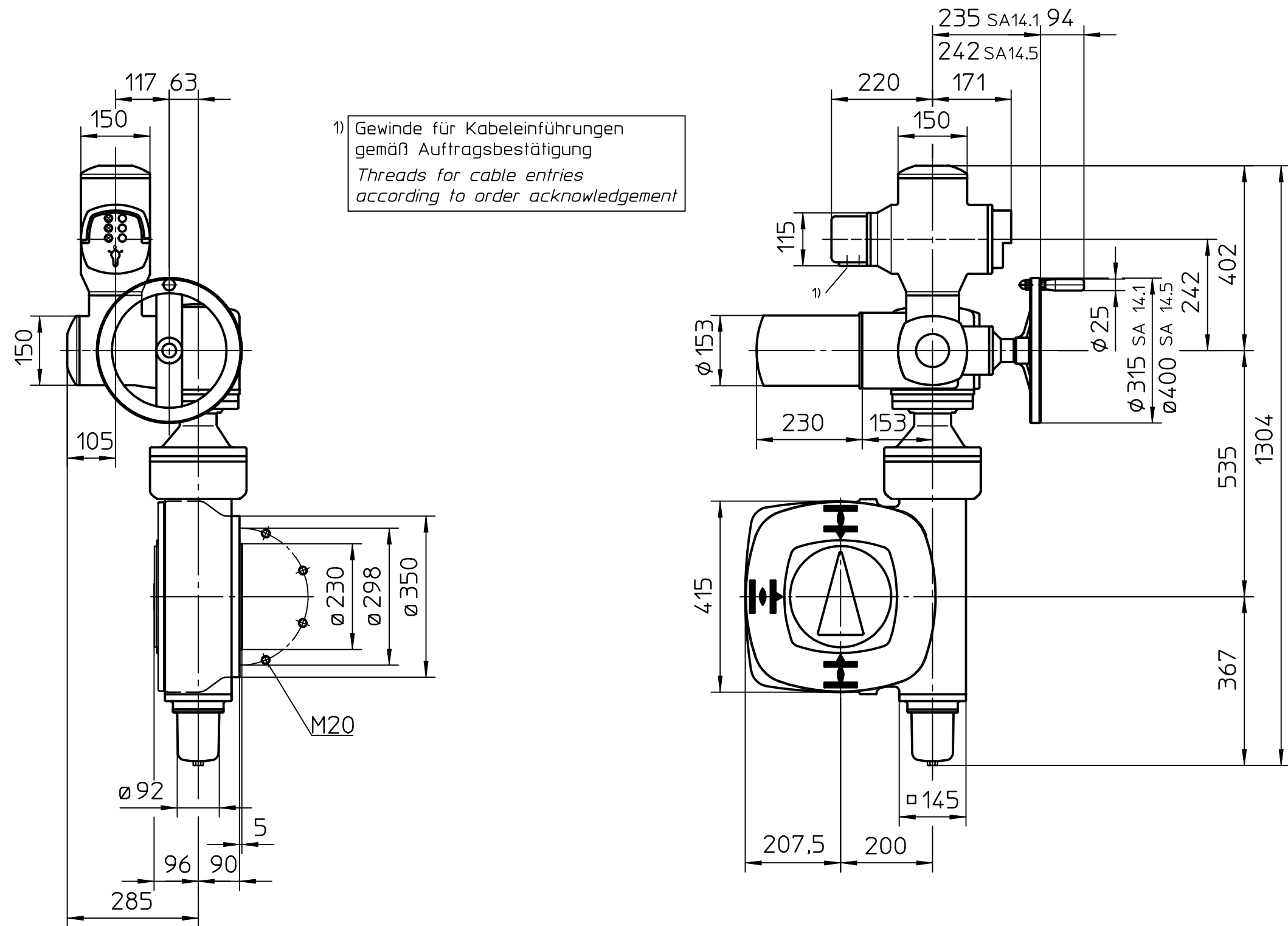
Montage-Position A/Mounting position A
