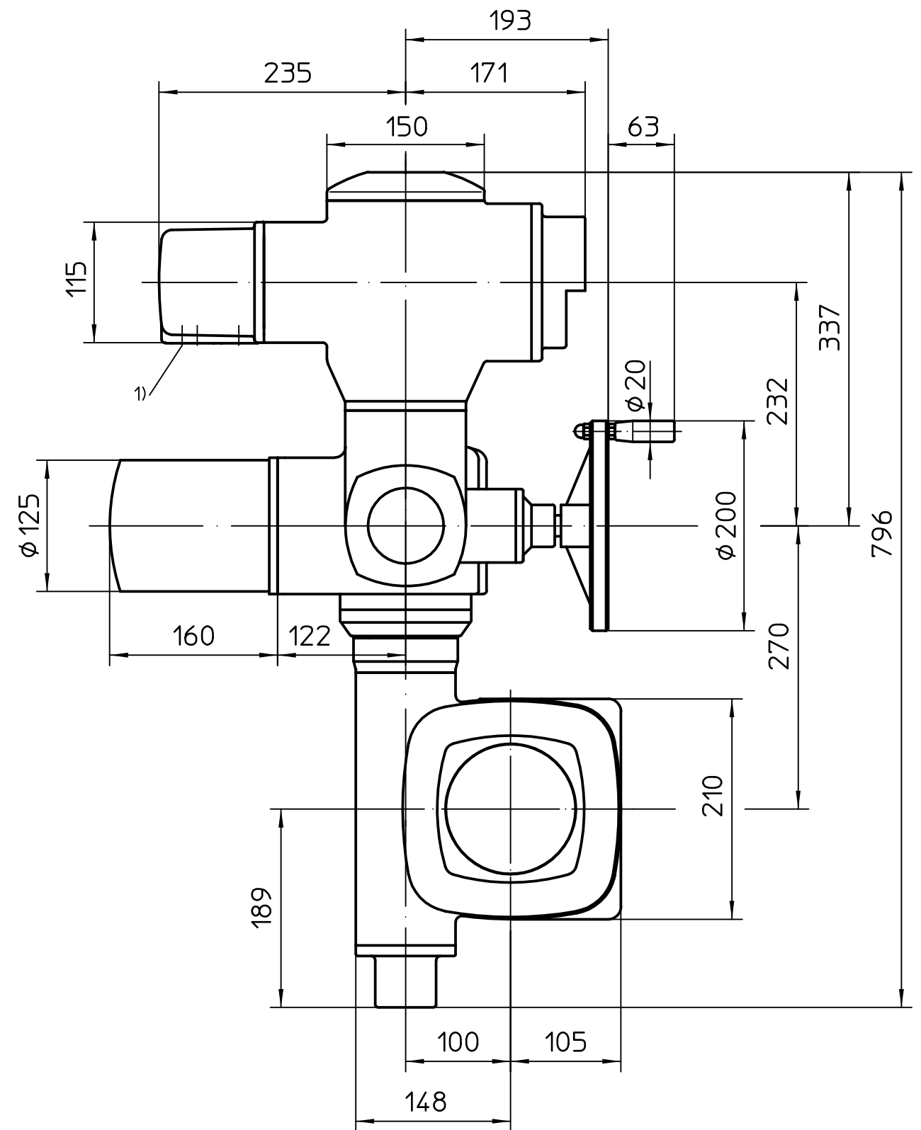
Montage-Position A/Mounting position A
