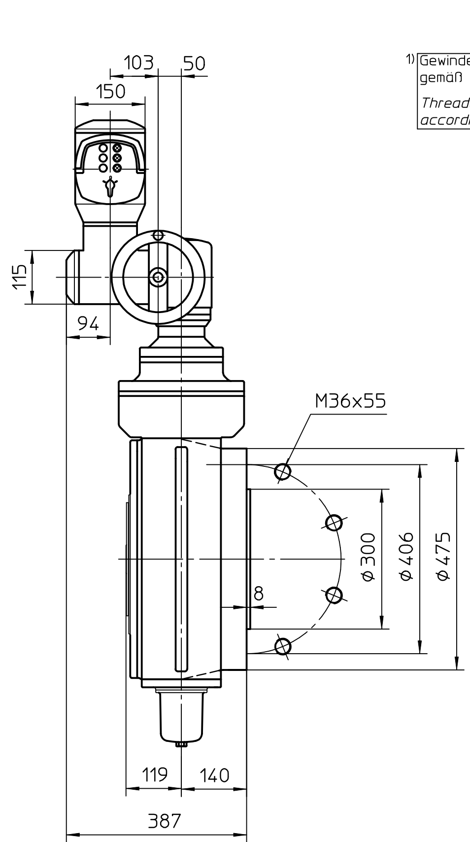
Montage-Position A/Mounting position A
