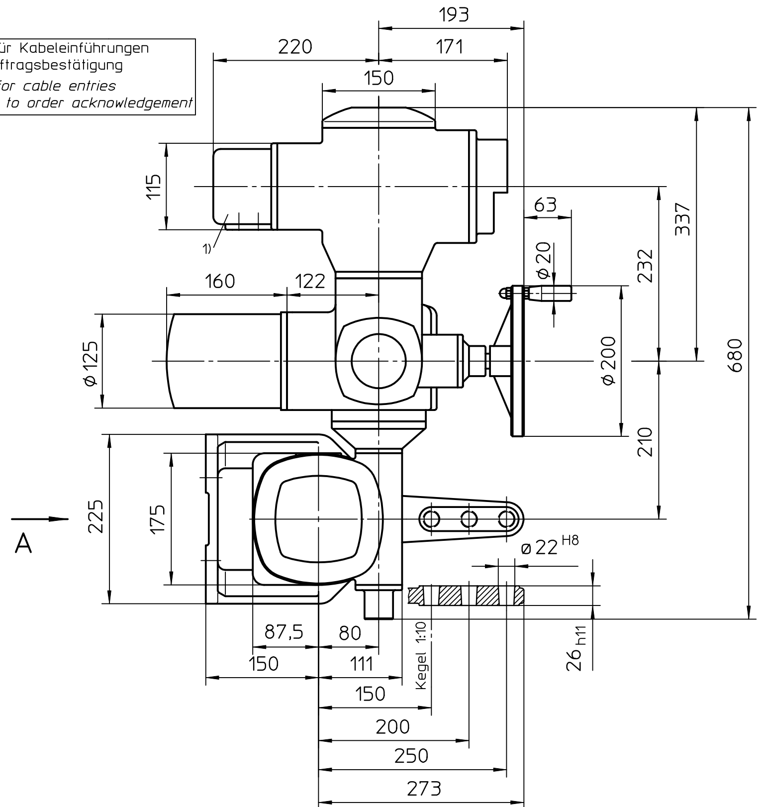
Montage-Position A/Mounting position A
