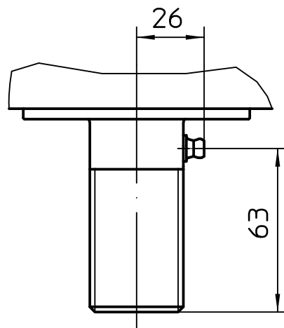
Detail X M 1:2
