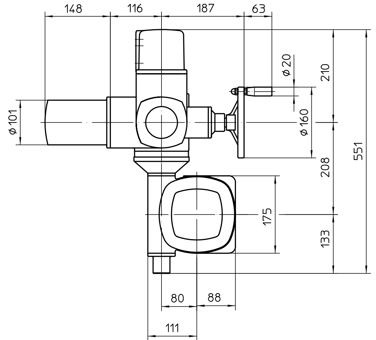
Montage-Position A/Mounting position A
