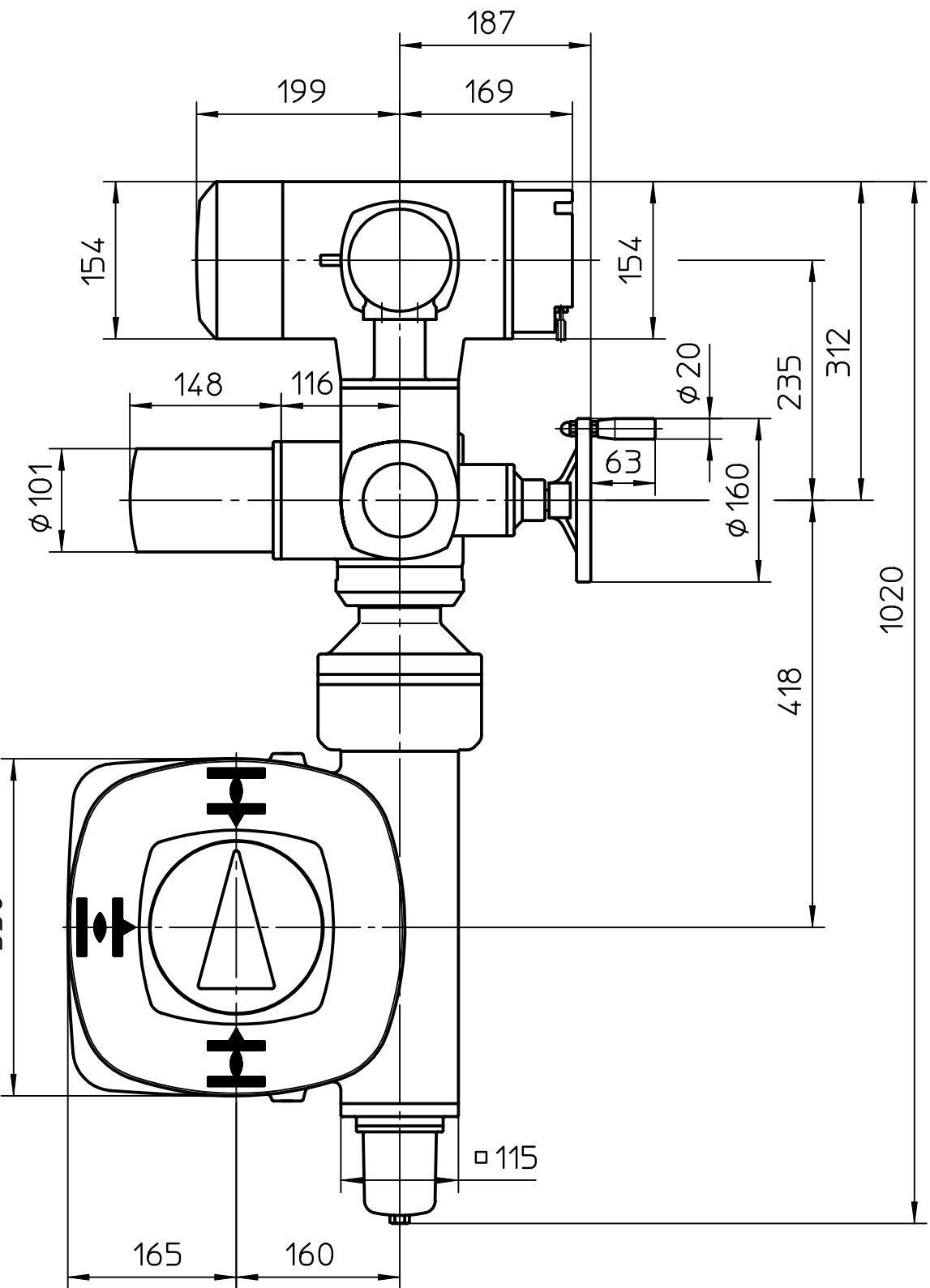
Montage-Position A/Mounting position A
