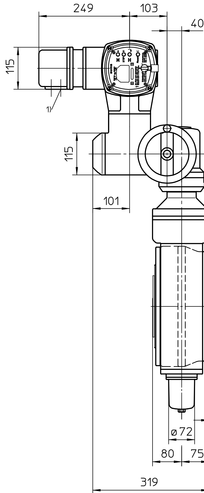
Standardversion KP Standard version KP
