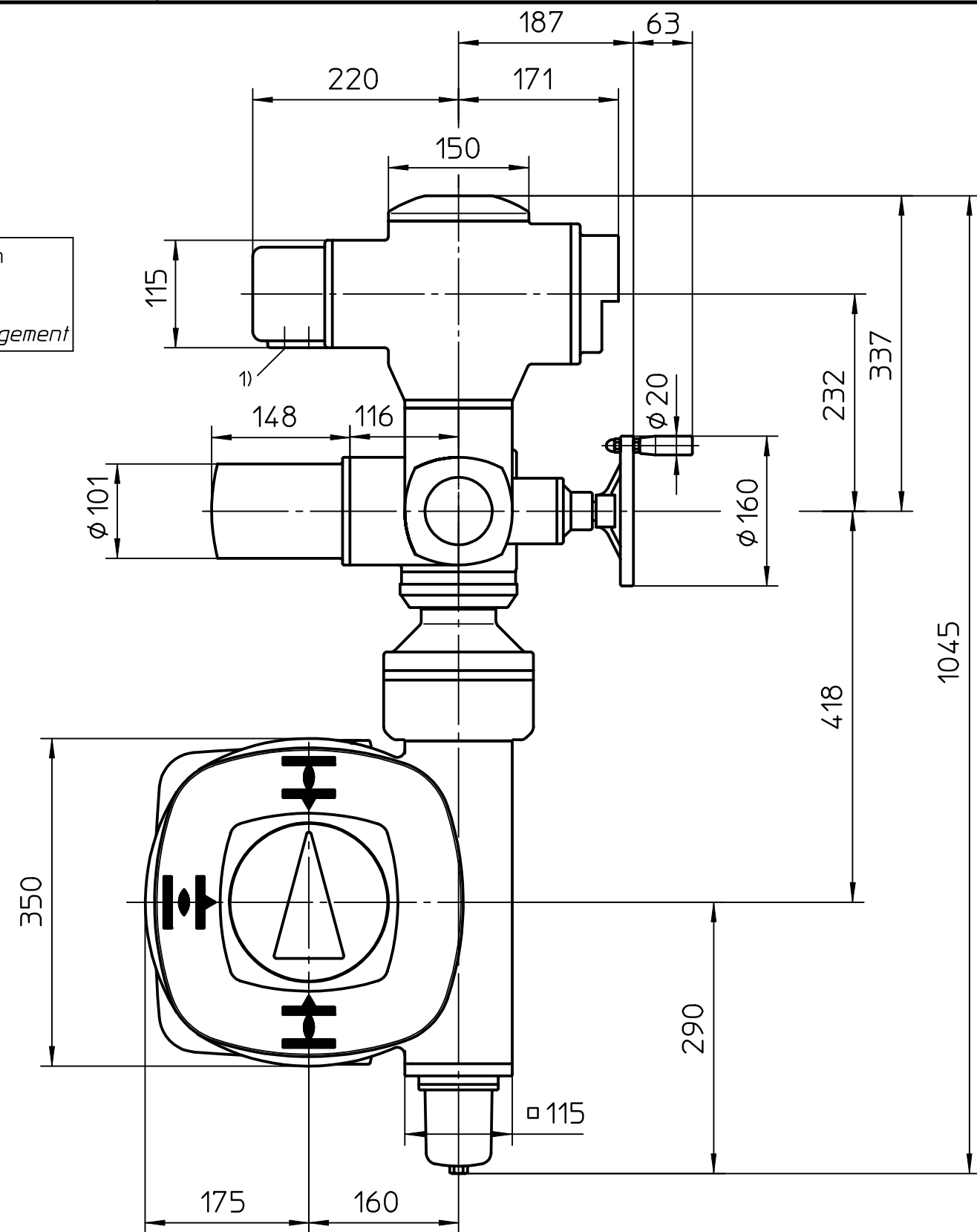
Montage-Position A/Mounting position A
