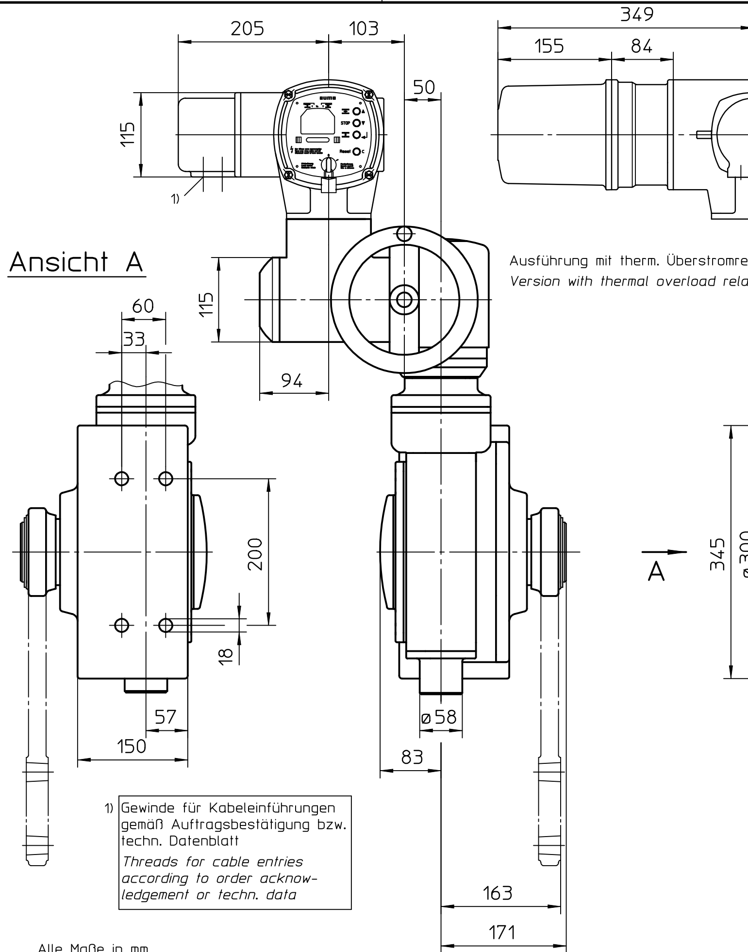
Montage-Position A/Mounting position A
