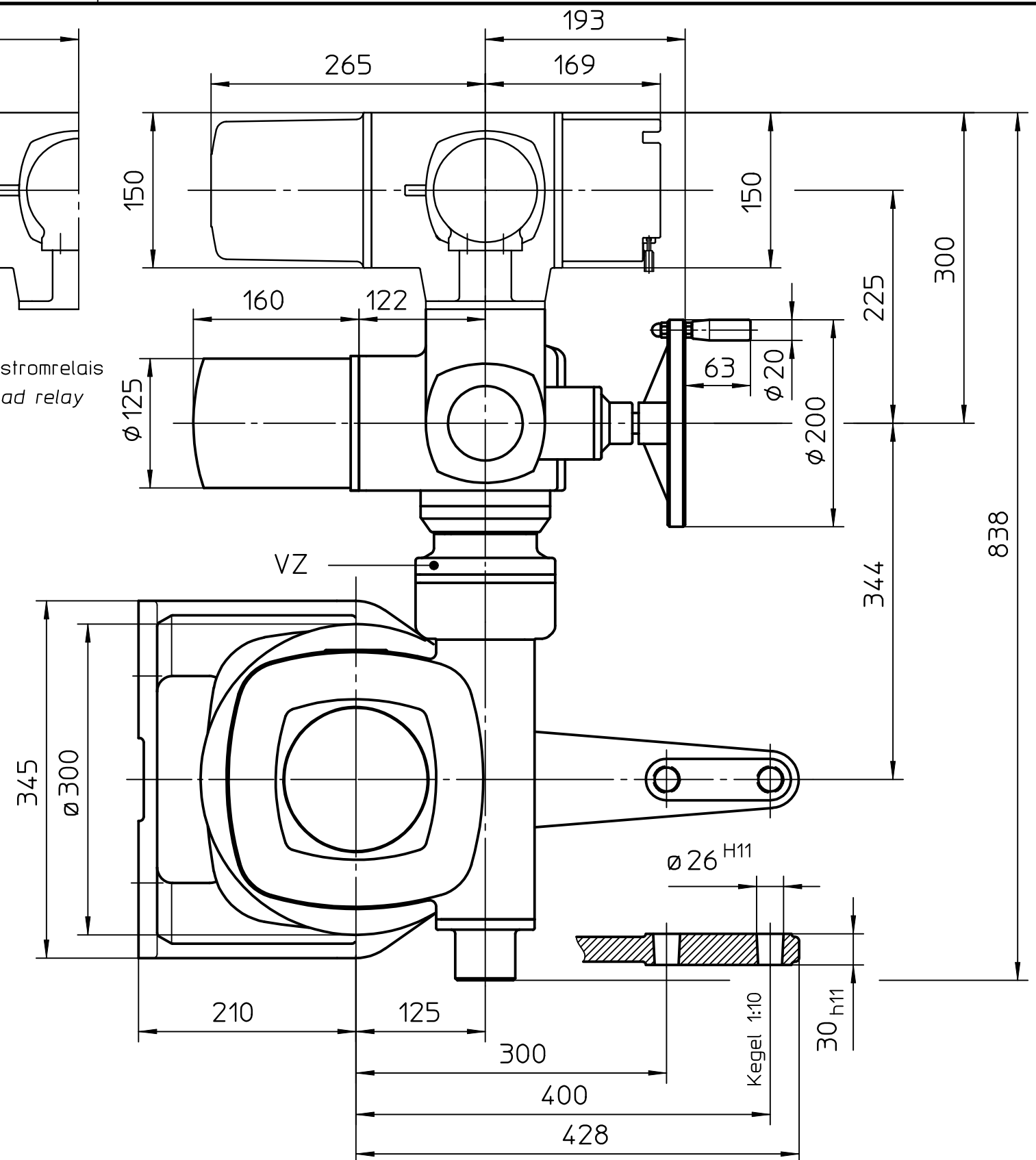
Montage-Position A/Mounting position A
