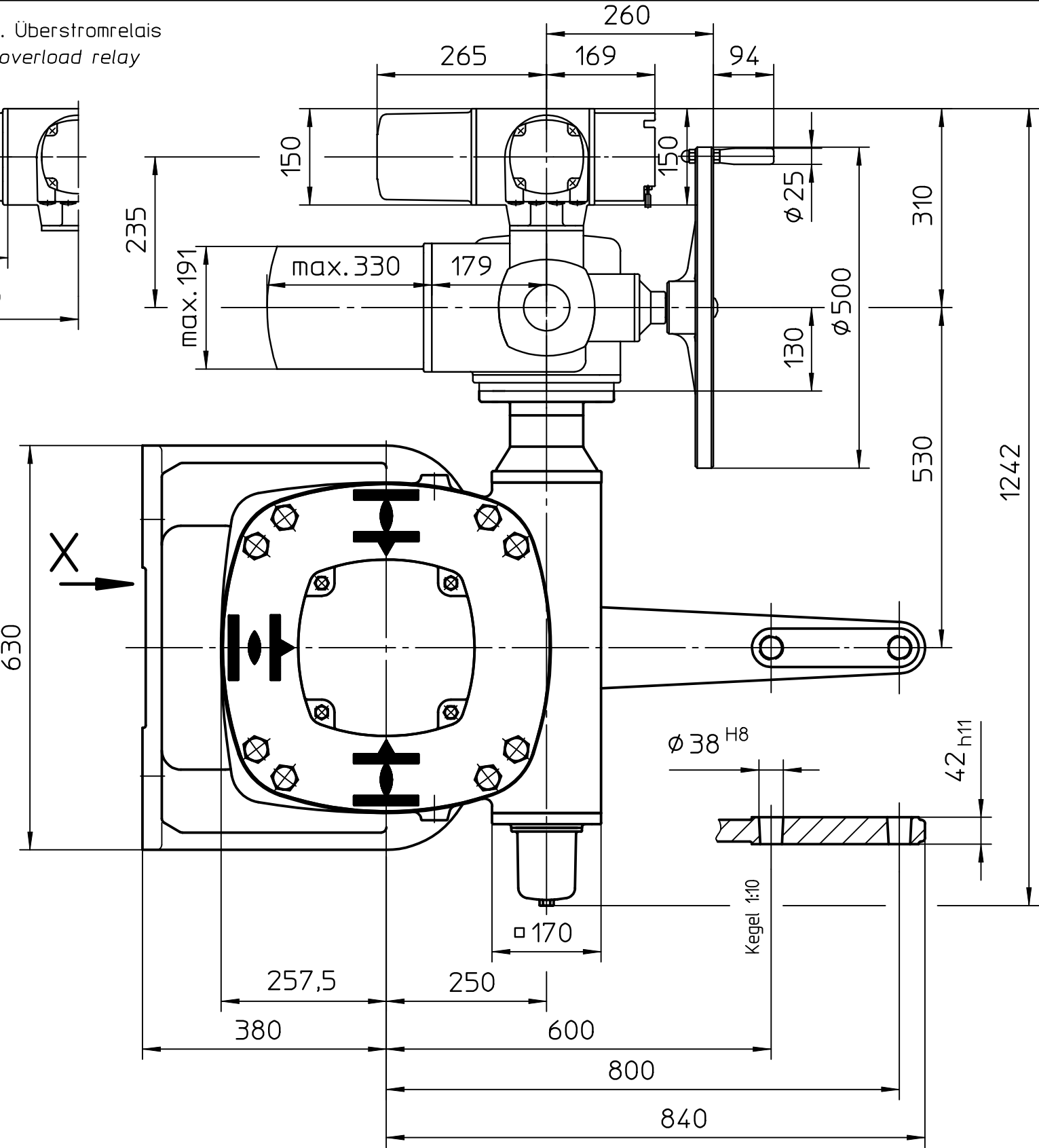
Montage-Position A/Mounting position A
