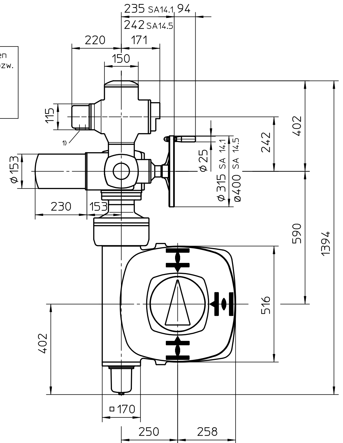
Montage-Position A/Mounting position A
