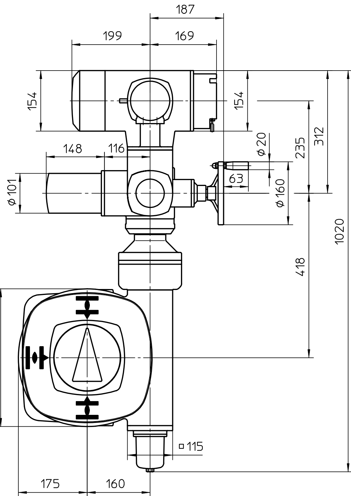
Montage-Position A/Mounting position A
