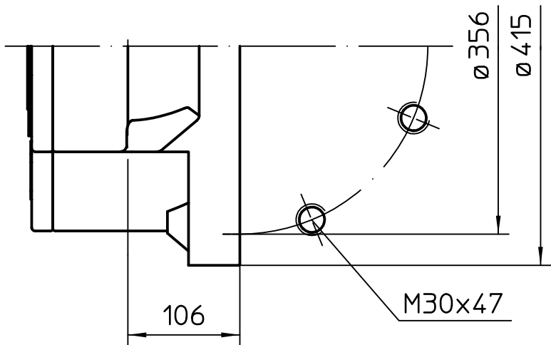
Option Flansch plan
