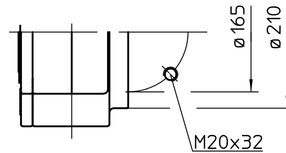
Option Flansch plan
