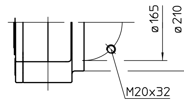
Option Flansch plan
