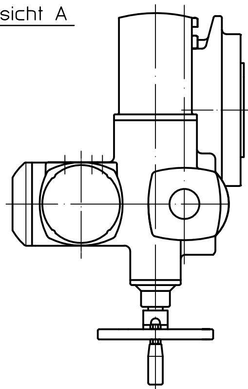
Option Flansch plan
