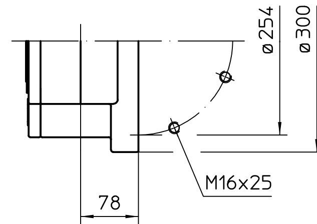
Option Flansch plan
