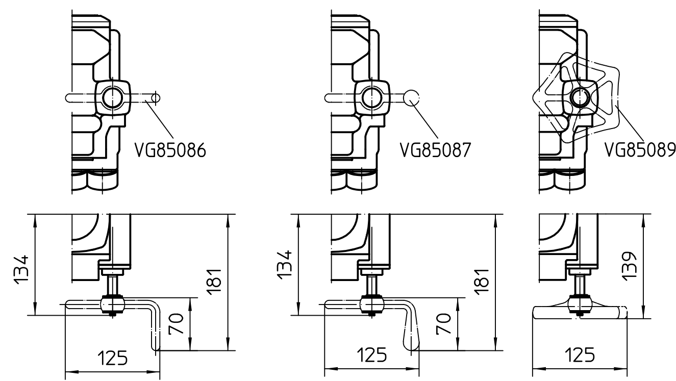
Possible variants (1:5)
