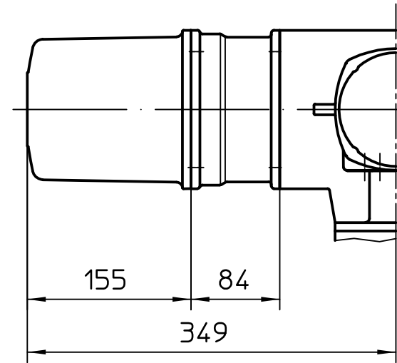
Version with thermal overload relay
