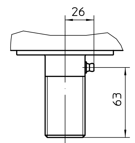
Detail X
