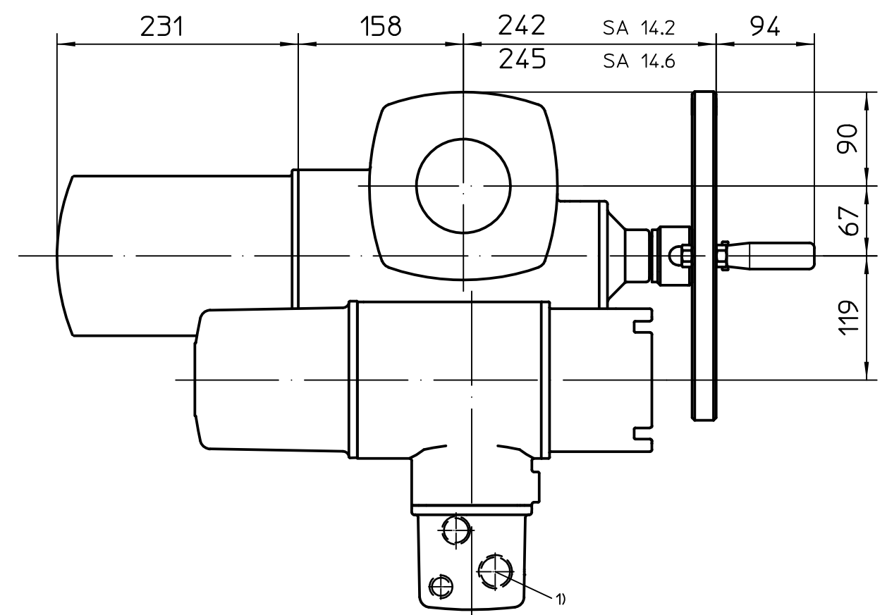
Version with thermal overload relay
