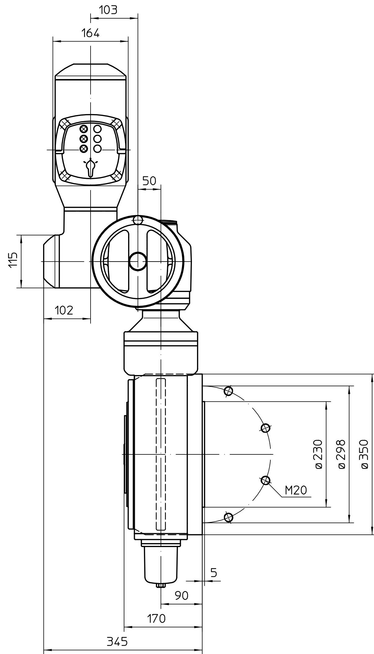
Plane flange option
