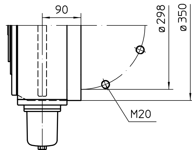
Plane flange option
