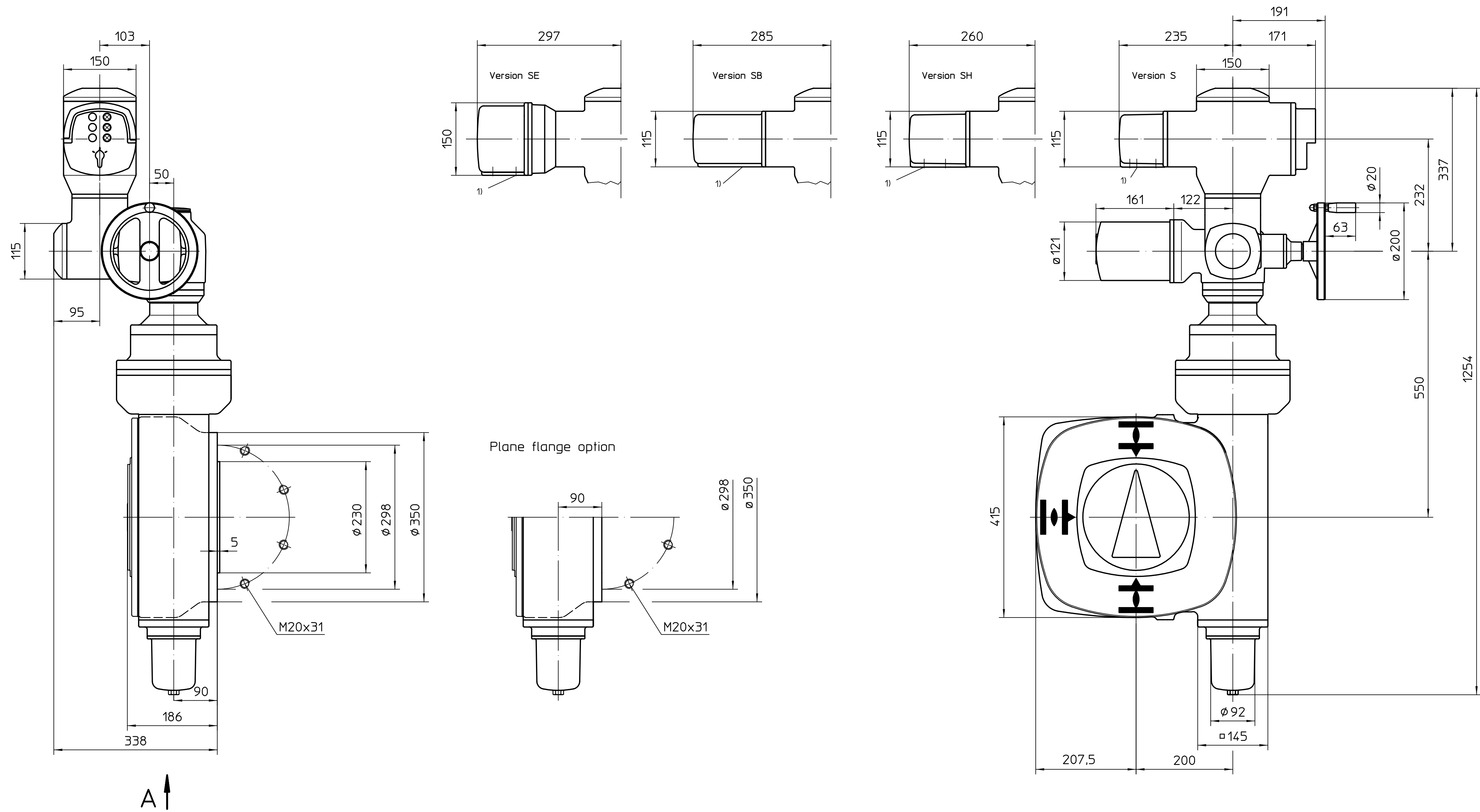
View A
