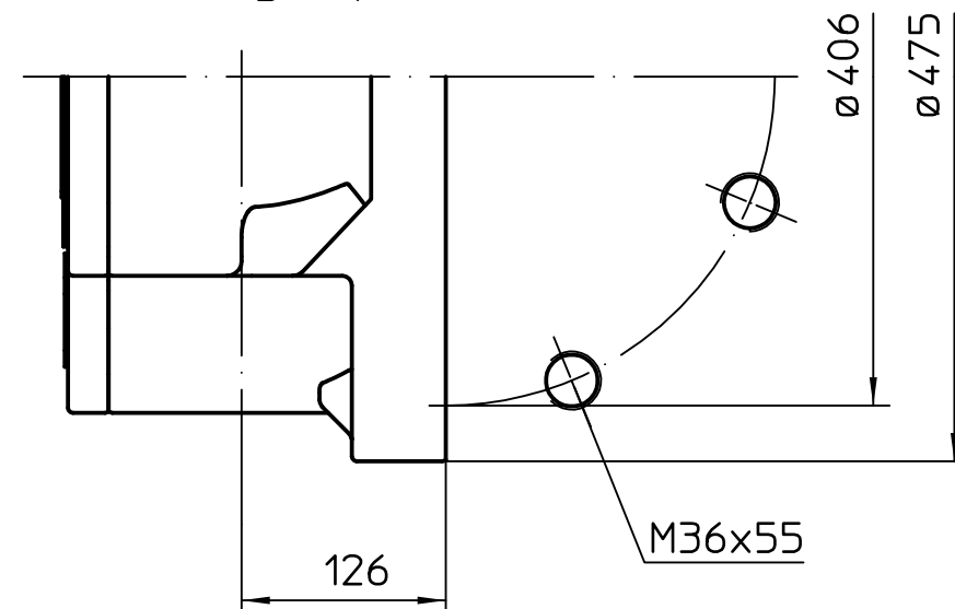
Plane flange option
