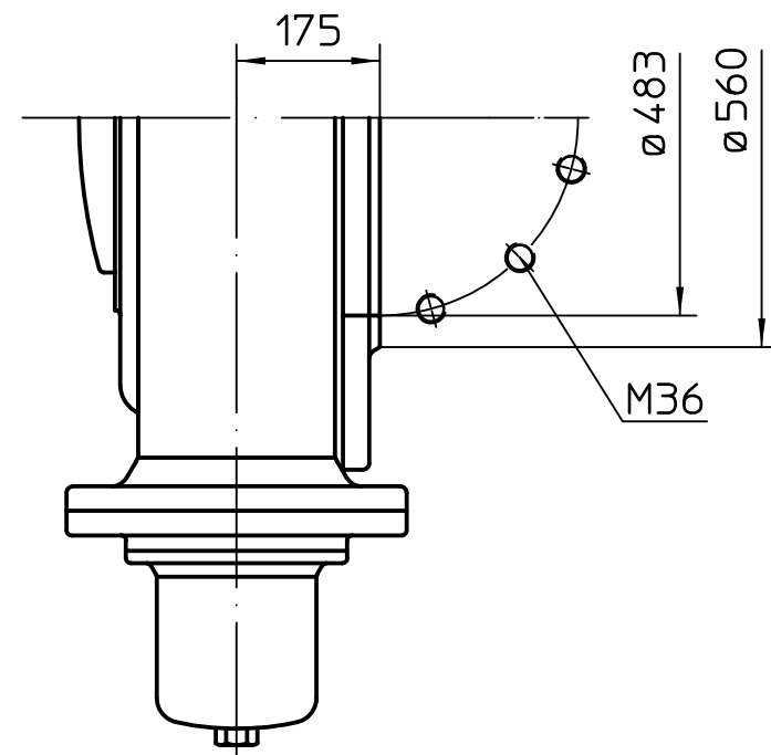
Plane flange option
