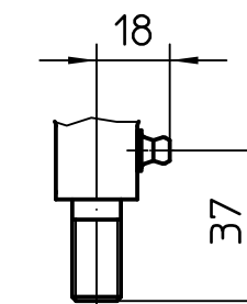
Detail X
