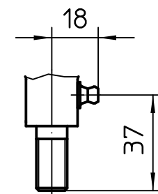
Detail X
