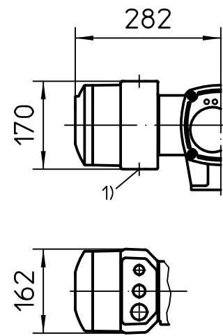
Version KT Exd Version KM Exd
