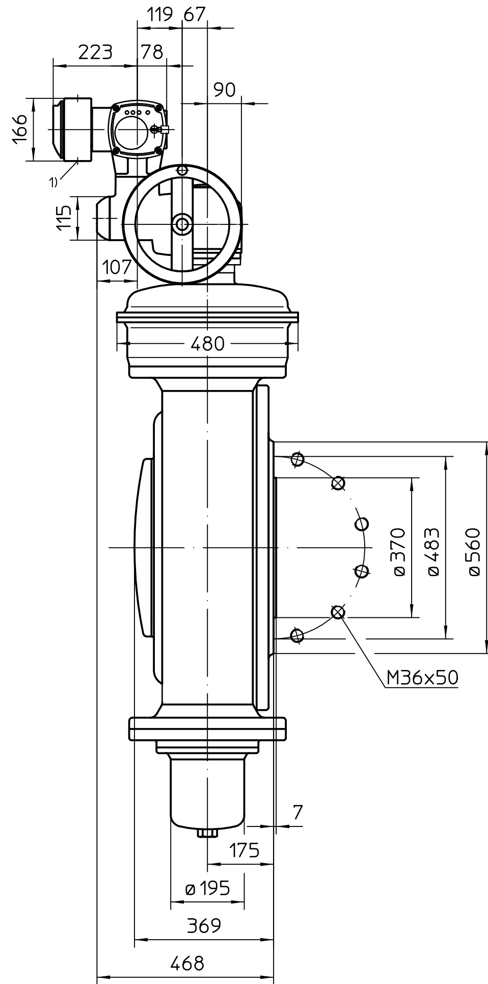
Standard version KT Exe
