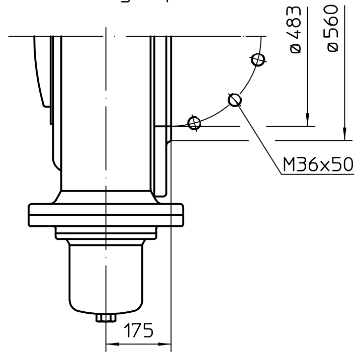
Plane flange option
