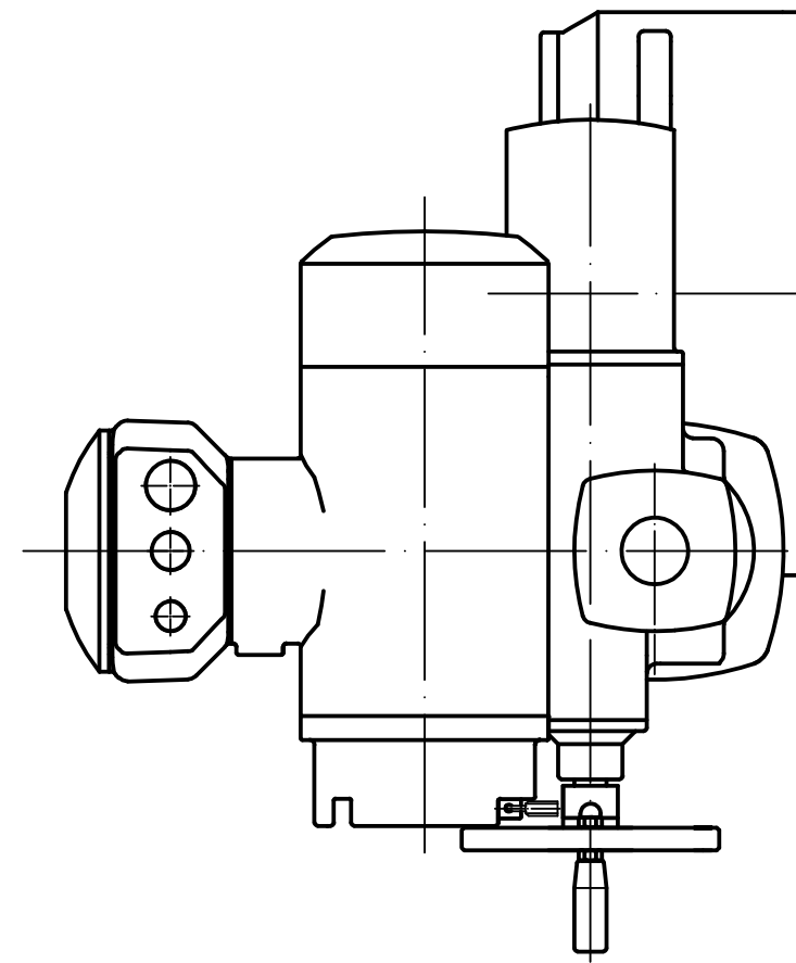
View A
