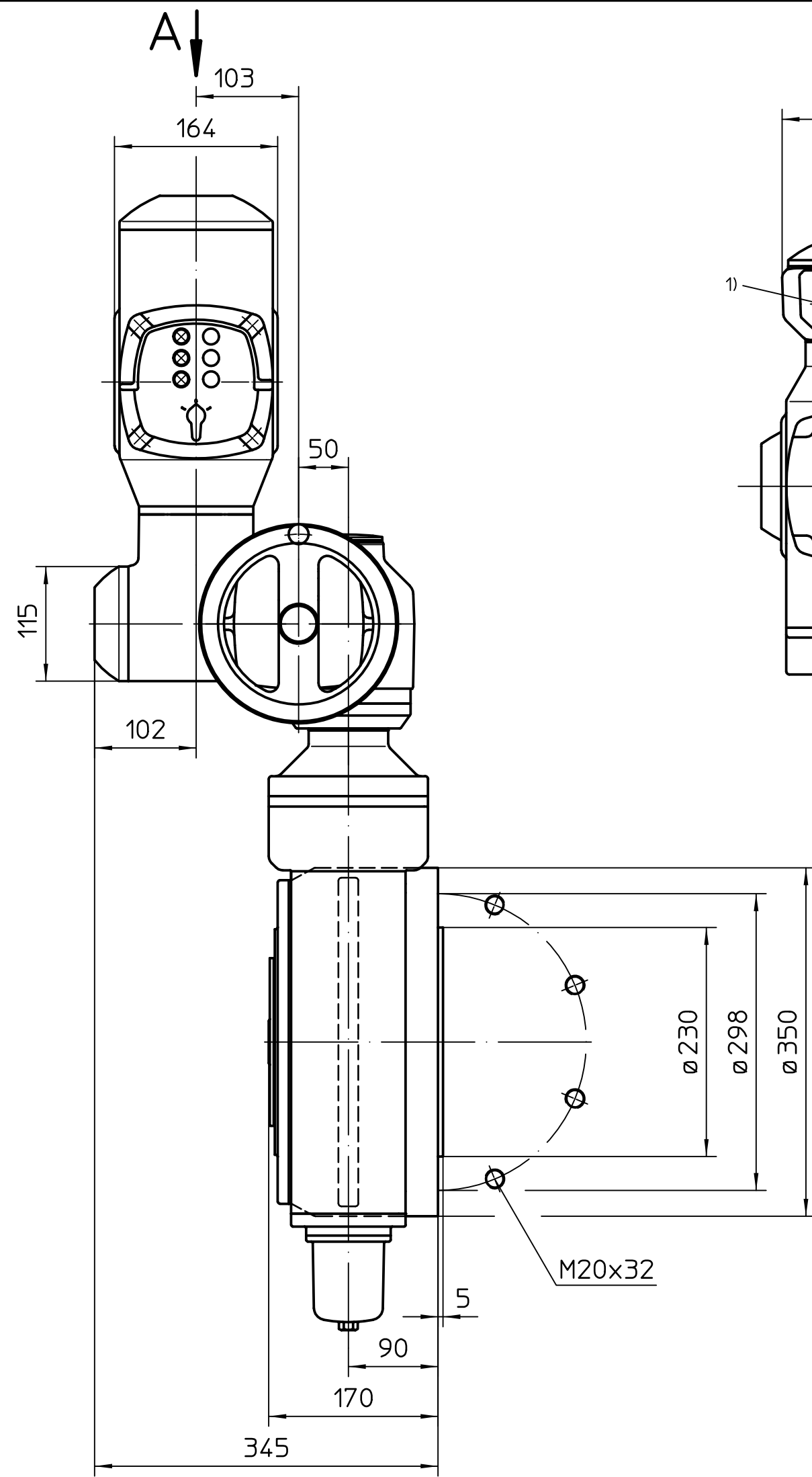
Plane flange option
