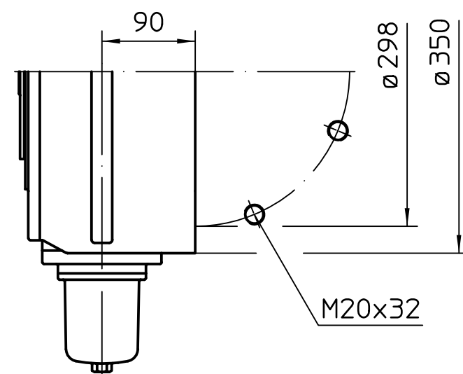
Plane flange option
